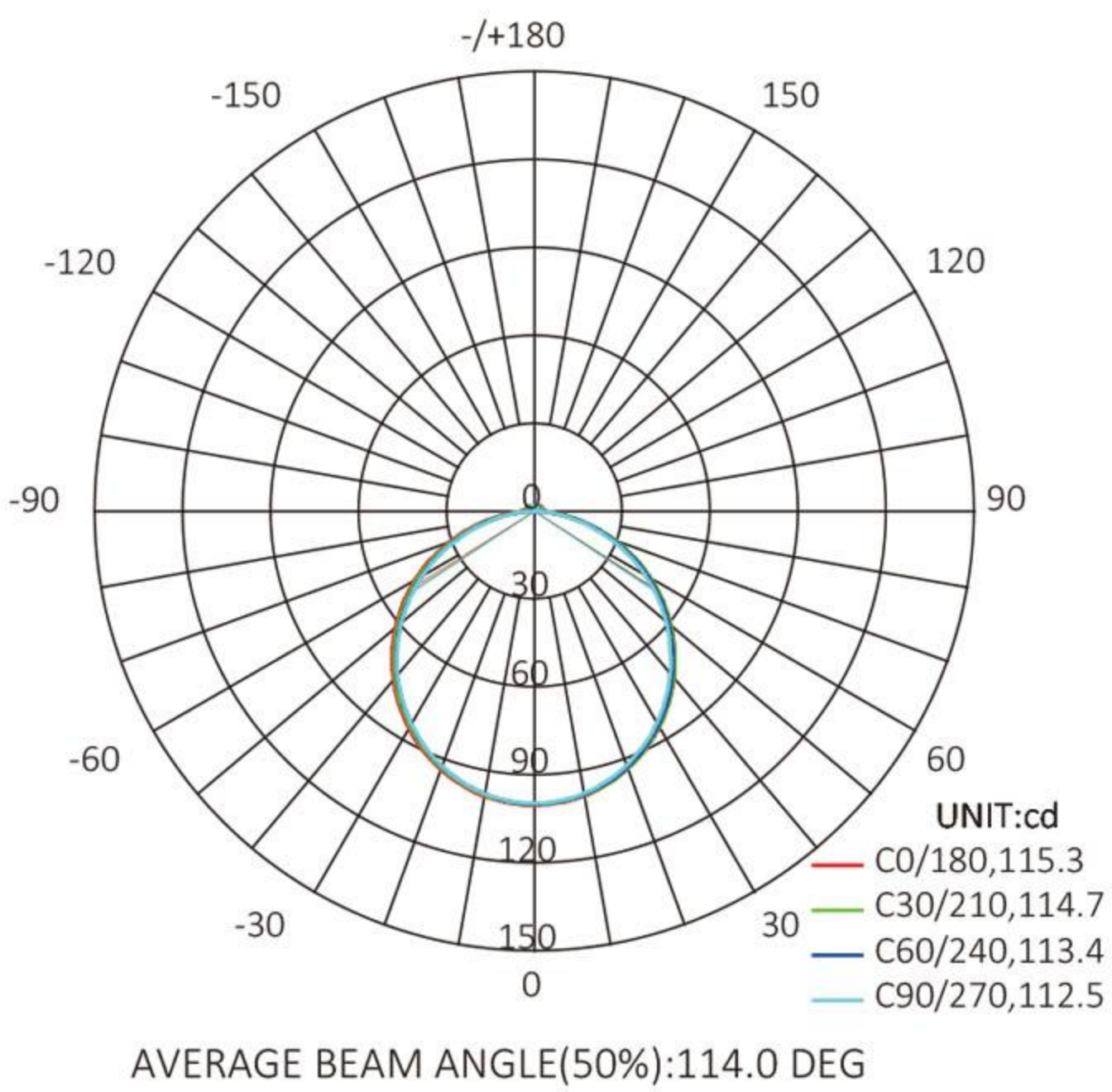
Luminous intensity distribution diagram
