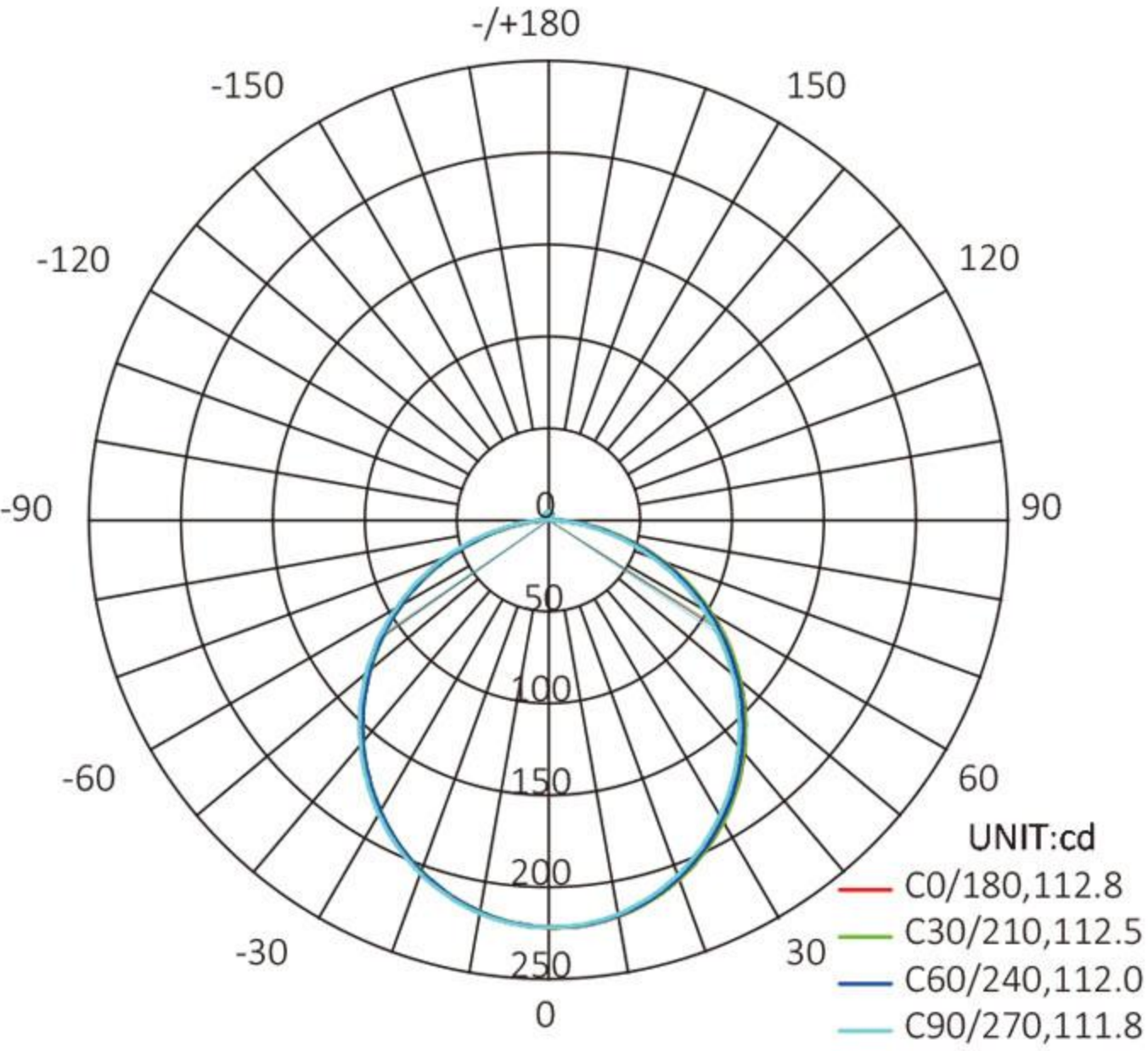
Luminous intensity distribution diagram
